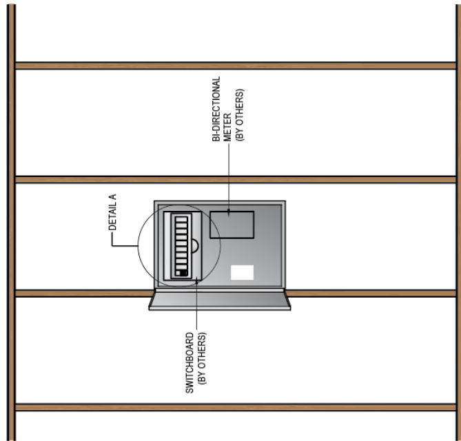
FRONT ELEVATION METER BOX LOCATION (FRAME STAGE)
