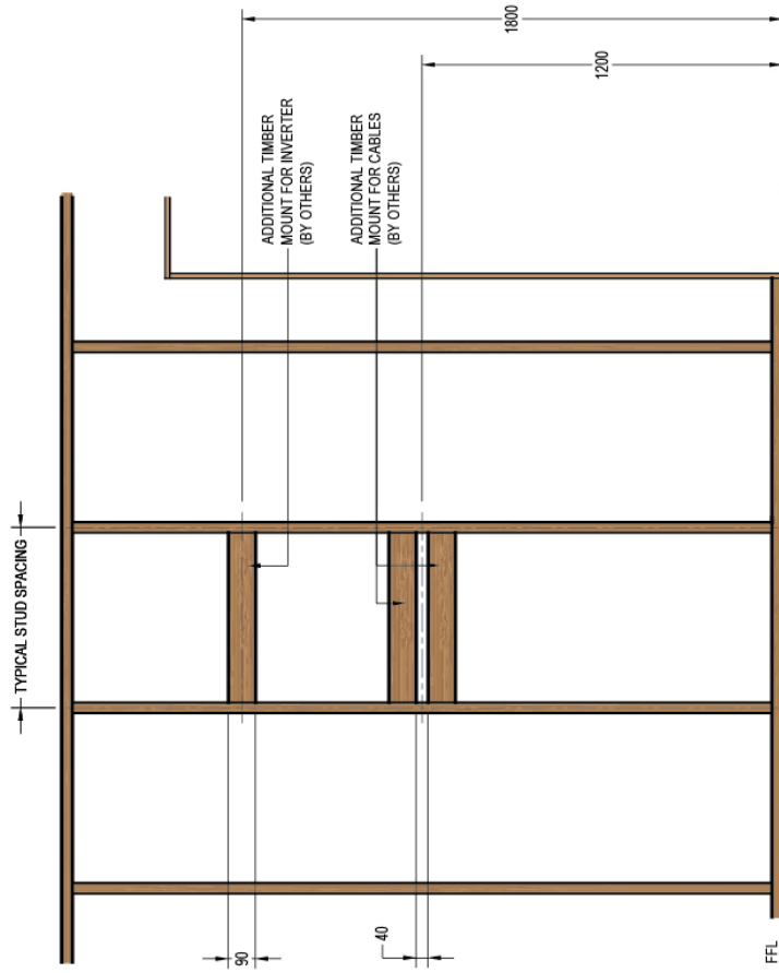
FRONT ELEVATION INVERTER LOCATION (FRAME STAGE)
